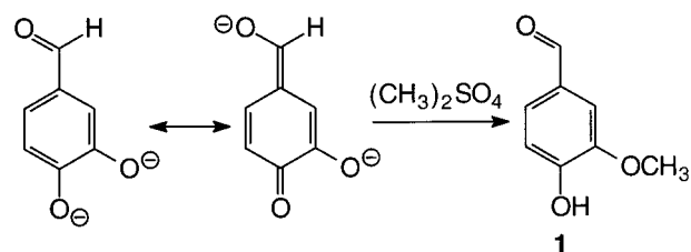
O=C(O)C(O)c1ccc(O)cc1 (14) \xrightarrow{+Cu^{++} / -Cu^{+}} OCC1=CC(=C(O)C(=C1)O (A) + CO_2 + H^{+} (a) OCC1=CC(=C(O)C(=C1)O (A) \xrightarrow{+Cu^{+} / -Cu^{+} / H^{+}} O=CC1=CC(=C(O)C(=C1)O (13) (b) OCC1=CC(=C(O)C(=C1)O (A) \xrightarrow{O_2} OCC1=CC(=C(O)C(=C1)O (B) B \rightleftharpoons O=CC1=CC(=C(O)C(=C1)O (13) \rightleftharpoons OCC1=CC(=C(O)C(=C1)O (C) C \xrightarrow{H_2O_2} O=CC1=CC(=C(O)C(=C1)O (13) 2 O=CC1=CC(=C(O)C(=C1)O (13) \rightarrow O=CC1=CC(=C(O)C(=C1)O (E) \rightarrow O=C(O)C(O)c1ccc(O)cc1 (17) O=C(O)C(O)c1ccc(O)cc1 (14) \rightleftharpoons O=CC1=CC(=C(O)C(=C1)O (13) + H_2O_2 H_2O_2 + 2 Cu(I) + 2 H^{+} \longrightarrow 2 Cu(II) + 2 H_2O
