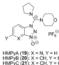
Figure 6. General structures of benzotriazole-based immonium salts containing pyrrolidino-morpholino systems.
