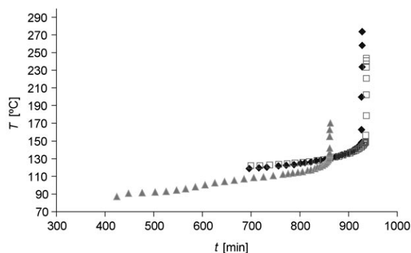
Figure 9. Decomposition profiles observed during ARC experiments with HDMB ( 8 , \square ), HDMA ( 7 , \blacklozenge ), and COMU ( 18c , \blacktriangle ) showing temperature ( ^{\circ}\text{C} ) as a function of time (min).
