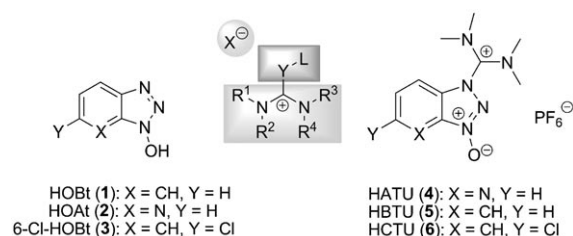
Figure 1. General structures of HOBt derivatives (left), immonium/uronium salts (center), and the most commonly used immonium salts (right).
