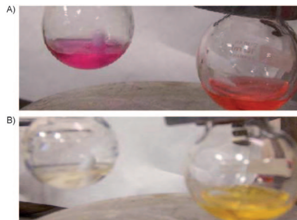
Figure 5. A) 2 min after the addition of COMU (pink with TMP and orange-red with DIEA). B) 1 h after the addition of COMU.
