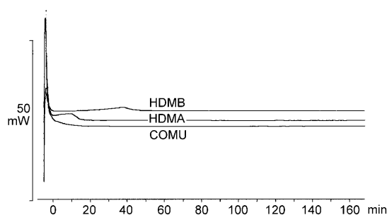
Figure 10. Thermograms showing heat flow versus time for isothermal DSC experiments set at 10^{\circ}\text{C} below the onset temperatures of HDMA ( 7 , 167^{\circ}\text{C} ), HDMB ( 8 , 170^{\circ}\text{C} ), and COMU ( 18c , 150^{\circ}\text{C} ).
