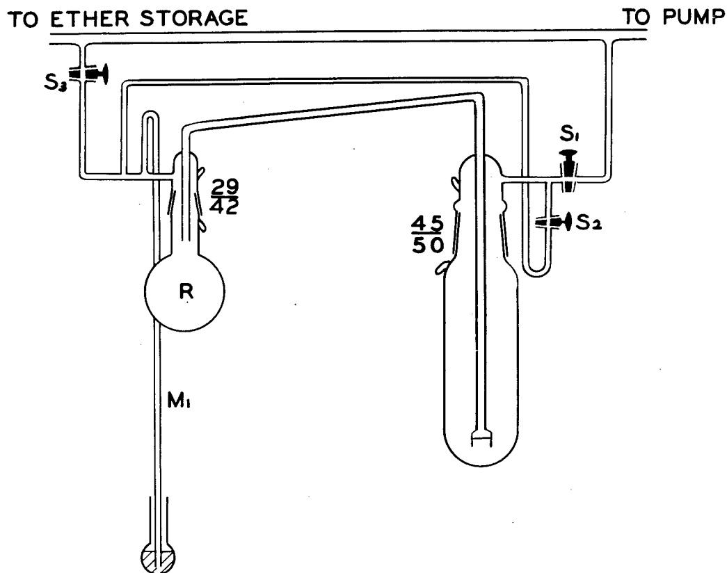
Figure 4. Apparatus for extraction of lithium borohydride.
