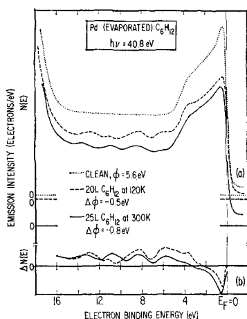
FIG. 1. Ultraviolet photoemission spectra at h\nu = 40.8 eV for (···) the clean polycrystalline Pd surface and for the same surface exposed to (---) 20 L of C_6H_{12} at 120°K and (—) 25 L of C_6H_{12} at 300°K. Spectra have been shifted vertically for clarity, as indicated by the position of zero marks. (b) Corresponding UPS difference curves for the (---) 120°K and (—) 300°K C_6H_{12} exposures to the clean polycrystalline Pd surface.
