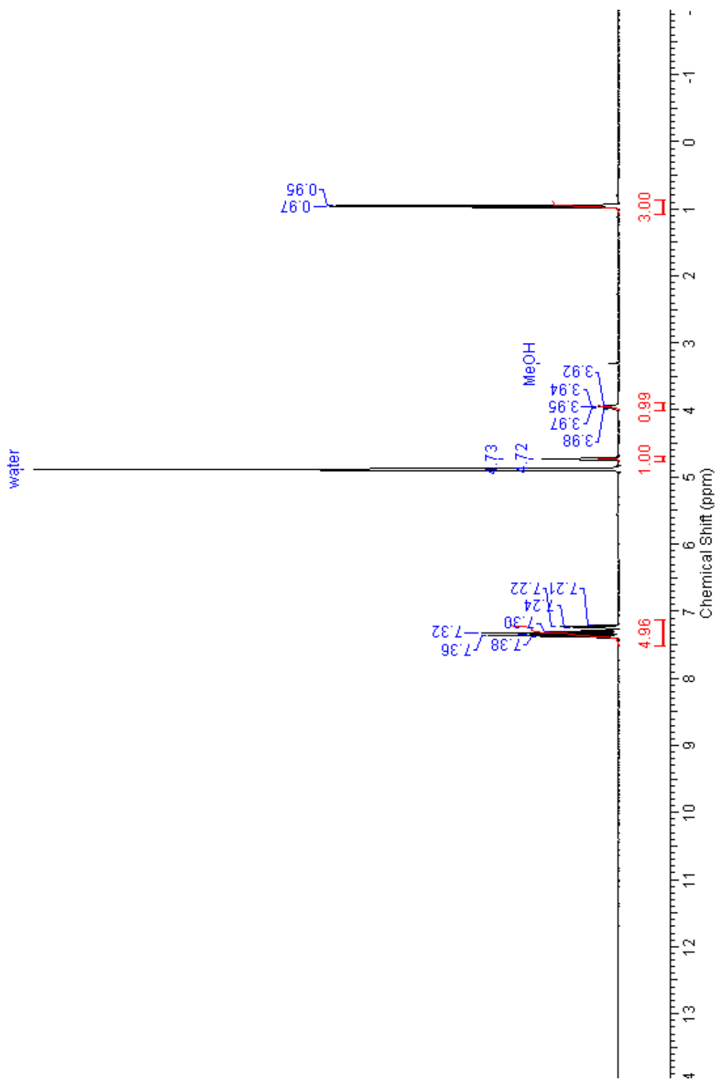
Figure 8. ^1\text{H} NMR, 8 scans, N-(2-Hydroxy-1-methyl-2-phenethyl)urea.
