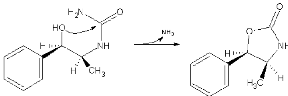
Figure 5. Formation of cis -4-Methyl-5-phenyl-1,3-oxazolidin-2-one from the Urea Intermediate.
