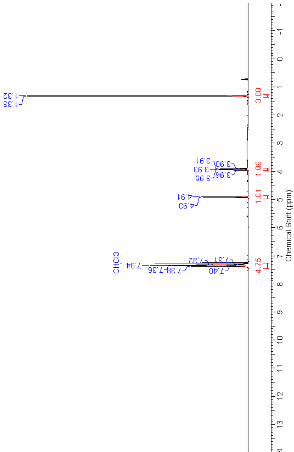
Figure 7. ^1\text{H} NMR, 8 scans, trans -4-Methylaminorex.
