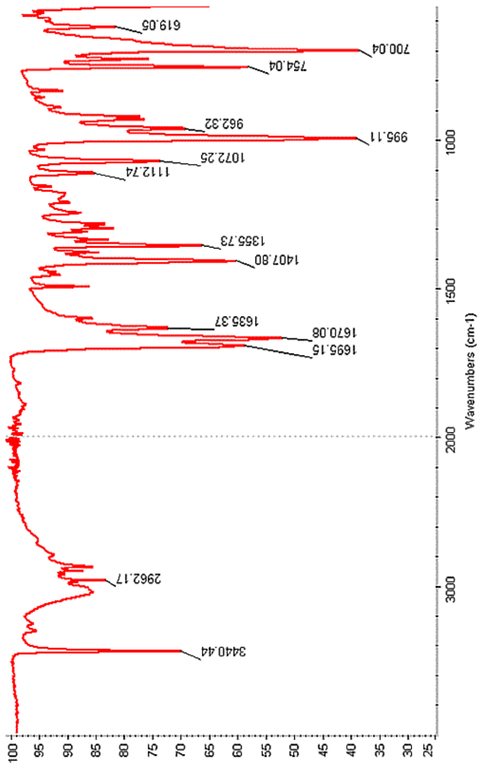
Figure 9. FTIR. 32 scans, trans -4-Methylaminorex.
