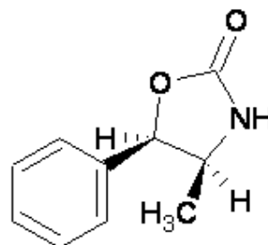
(4 S ,5 R )-4-methyl-5-phenyl-1,3-oxazolidin-2-one
