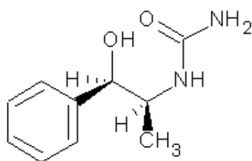
N-[(1 S ,2 R )-2-hydroxy-1-methyl-2-phenylethyl]urea
