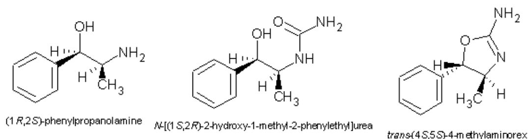
Figure 4. Summary of Absolute Configurations of Chiral Centers of Key Molecules. One of Each Enantiomeric Pair Is Shown.
