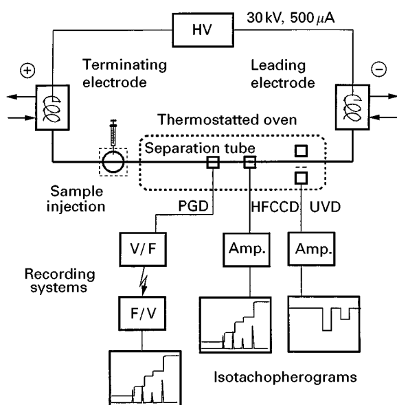
Figure 3 ITP apparatus with potential gradient detection (PGD), high-frequency contactless conductivity detection (HFCCD), and ultraviolet detection (UVD). HV, high-voltage power supply (constant current); V/F, voltage-frequency converter; F/V, frequency-voltage converter.
