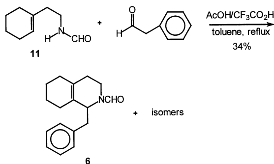
Scheme 4. Synthesis of isomeric octahydroisoquinolines 6 from N -[2-(cyclohex-1-enyl)ethyl]formamide
