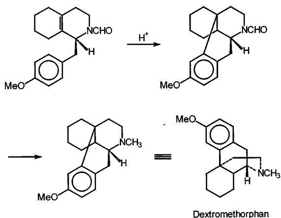
Scheme 1. Synthesis of dextromethorphan from (1 S )-1-( p -methoxybenzyl)- N -formyl-1,2,3,4,5,6,7,8-octahydroisoquinoline
