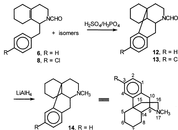
Scheme 5. Synthesis of morphinans from the isomeric octahydroisoquinolines
