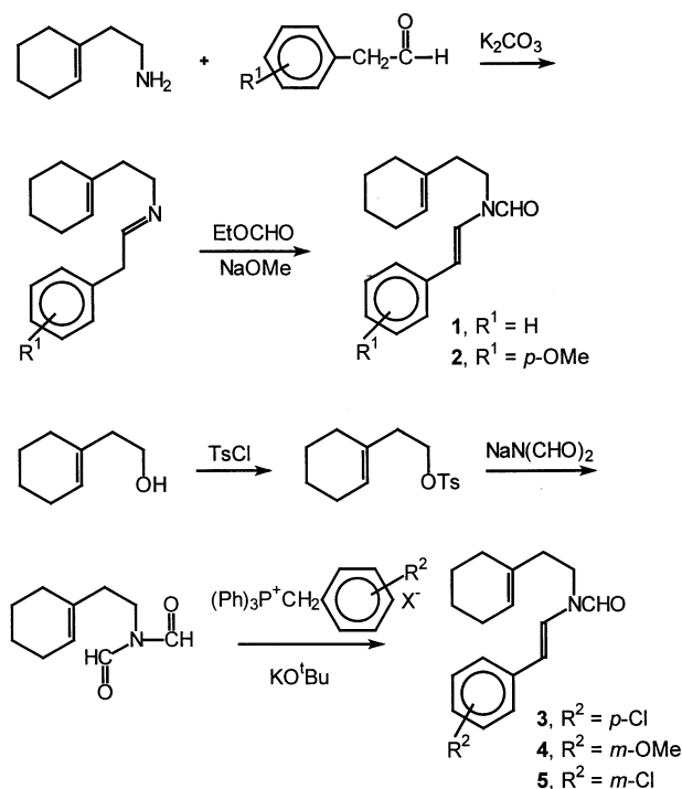
Scheme 2. Two synthetic pathways to substituted N -[2-(cyclohex-1-enyl)ethyl]- N -styrylformamides 1–2 and 3–5
