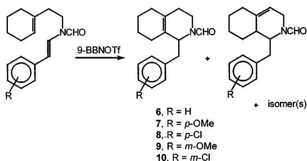
Scheme 3. Synthesis of phenyl-substituted N -[2-(cyclohex-1-enyl)ethyl]- N -styrylformamides
