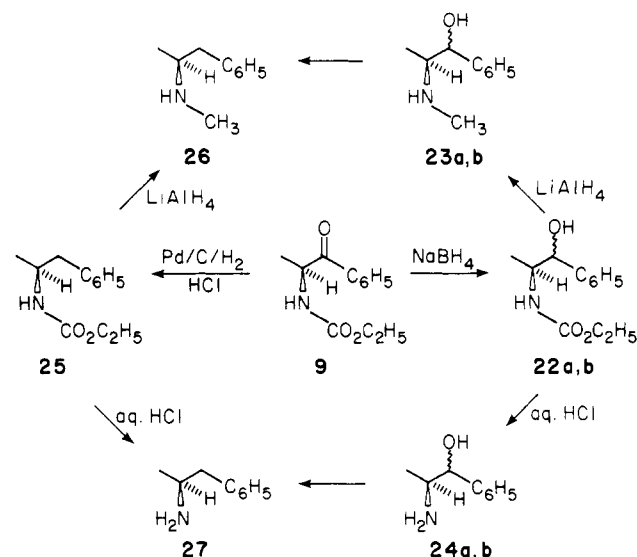
Scheme I. Reduction of ( S )-2-((Ethoxycarbonyl)amino)-1-phenyl-1-propanone to Ephedrine, Pseudoephedrine, and Amphetamines
