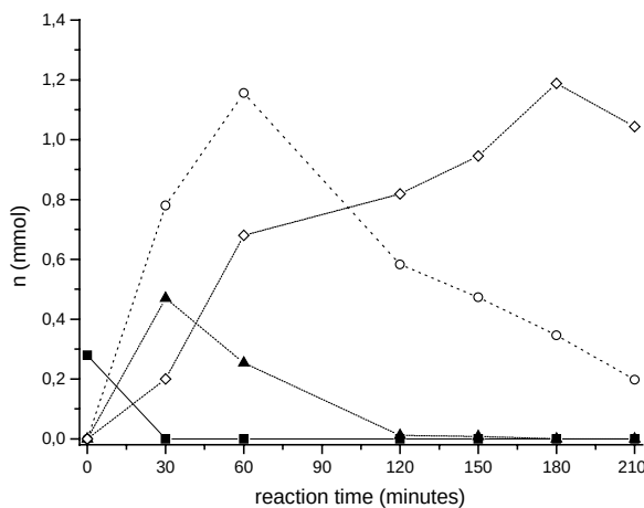
Fig. 3. Conversion of 1-phenyl-1,2-propanedione ( 1 ) (■) to (R)-1-hydroxy-1-phenyl-2-propanone ( 2 ) (○), (1R,2S)-1-phenyl-1,2-propanediol ( 3 ) (◇) and (S)-2-hydroxy-1-phenyl-1-propanone ( 4 ) (▲) mediated by pre-treated baker's yeast with nitrogen (60 min) followed by oxygen (20 min).
