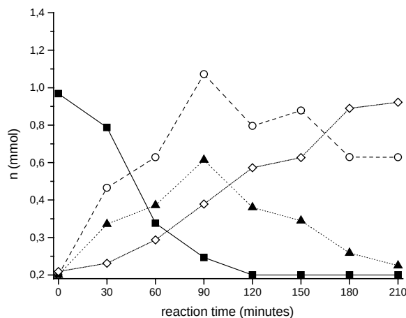
Fig. 1. Anaerobic process. Conversion of 1-phenyl-1,2-propanedione ( 1 ) (■) to (R)-1-hydroxy-1-phenyl-2-propanone ( 2 ) (○), (1R,2S)-1-phenyl-1,2-propanediol ( 3 ) (◇) and (S)-2-hydroxy-1-phenyl-1-propanone ( 4 ) (▲) mediated by anaerobically pre-treated baker's yeast.
