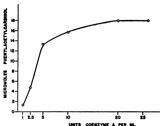
Figure 1. Effect of coenzyme A concentration on synthesis of phenylacetylcarbinol. Acetone powder, 5 mg; pyruvic acid, 48 \mu M; benzaldehyde, 18 \mu M; \text{MgSO}_4 , 13 \mu M; diphosphothiamin, 0.8 mg; diphosphopyridine nucleotide, 1.6 mg; M/15 phthalate buffer, pH 5.5, 0.7 ml; coenzyme A, as indicated. Final volume, 4.2 ml; 28 C; 90 minutes.
