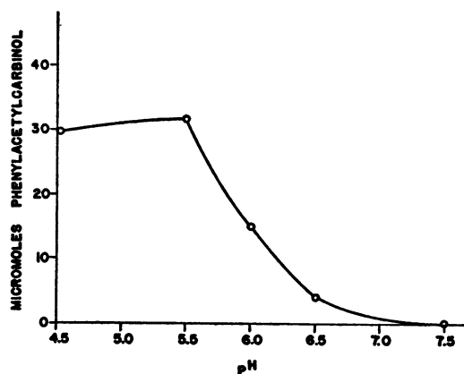
Figure 2. Effect of pH on the formation of phenylacetylcarbinol. Acetone powder, 5 mg; acetyl phosphate, 50 \mu\text{M} ; benzaldehyde, 50 \mu\text{M} ; coenzyme A, 100 U; \text{MgSO}_4 , 26 \mu\text{M} ; buffers as indicated in text. Total volume, 4.0 ml. Reaction time and temperature: 45 minutes at 28 C.
