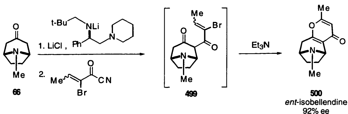
Scheme 86
