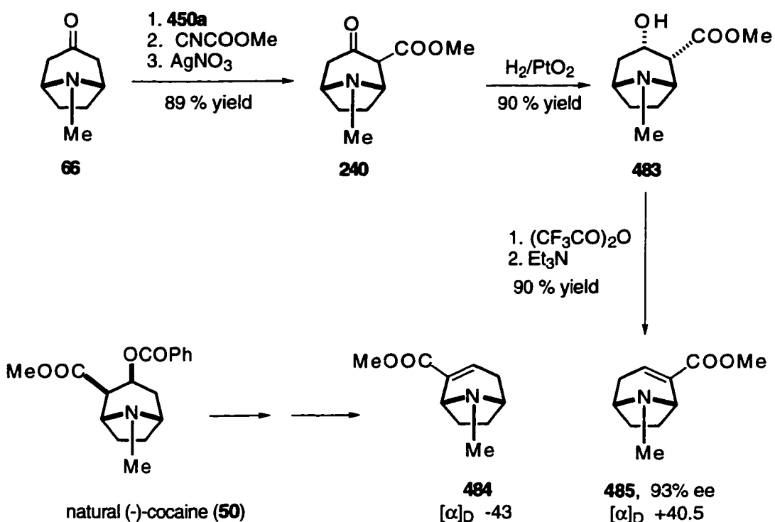
Scheme 79
