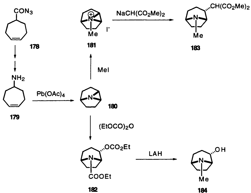
Scheme 33
