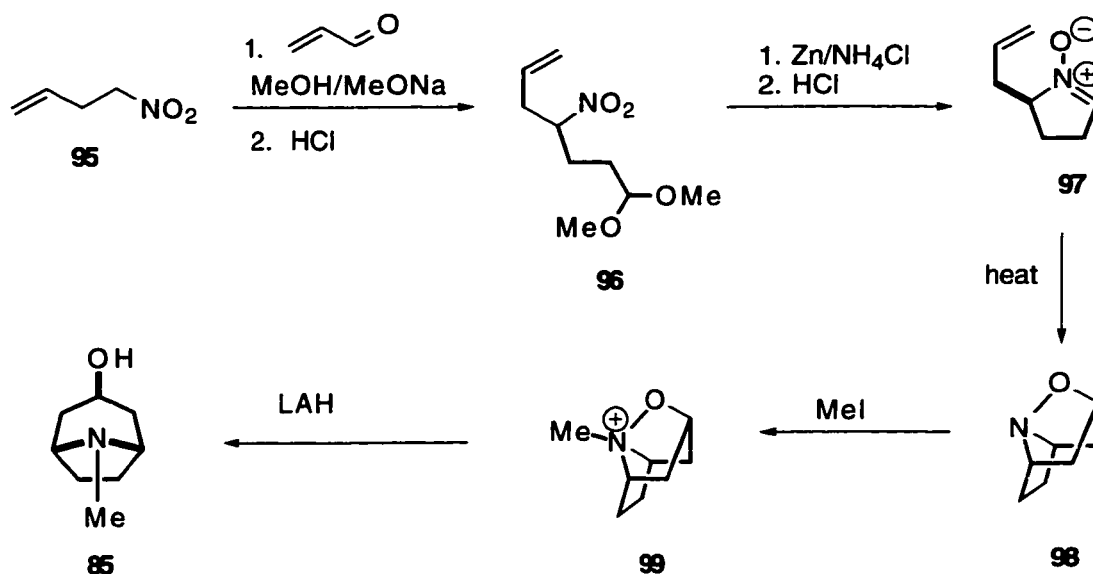
Scheme 19
