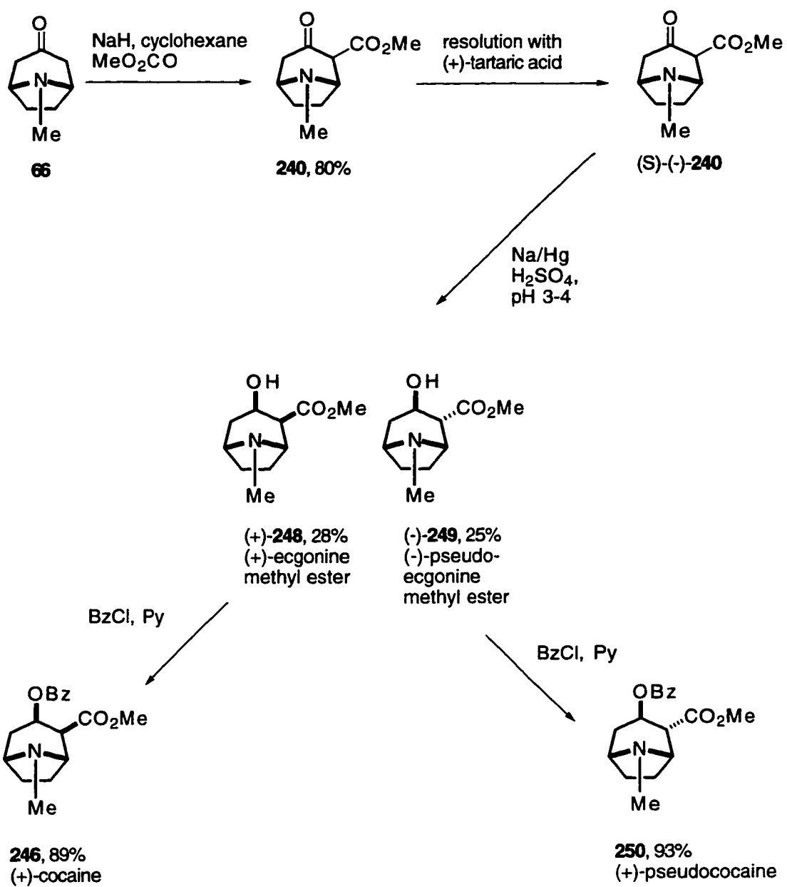
Scheme 45
