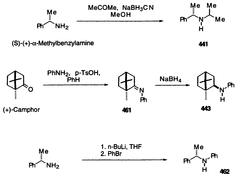
Scheme 69
