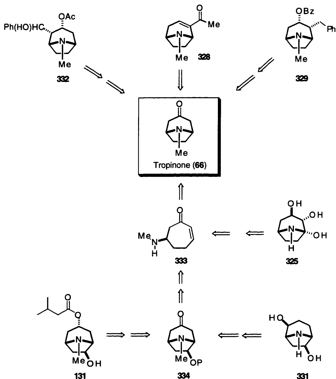
Scheme 63
