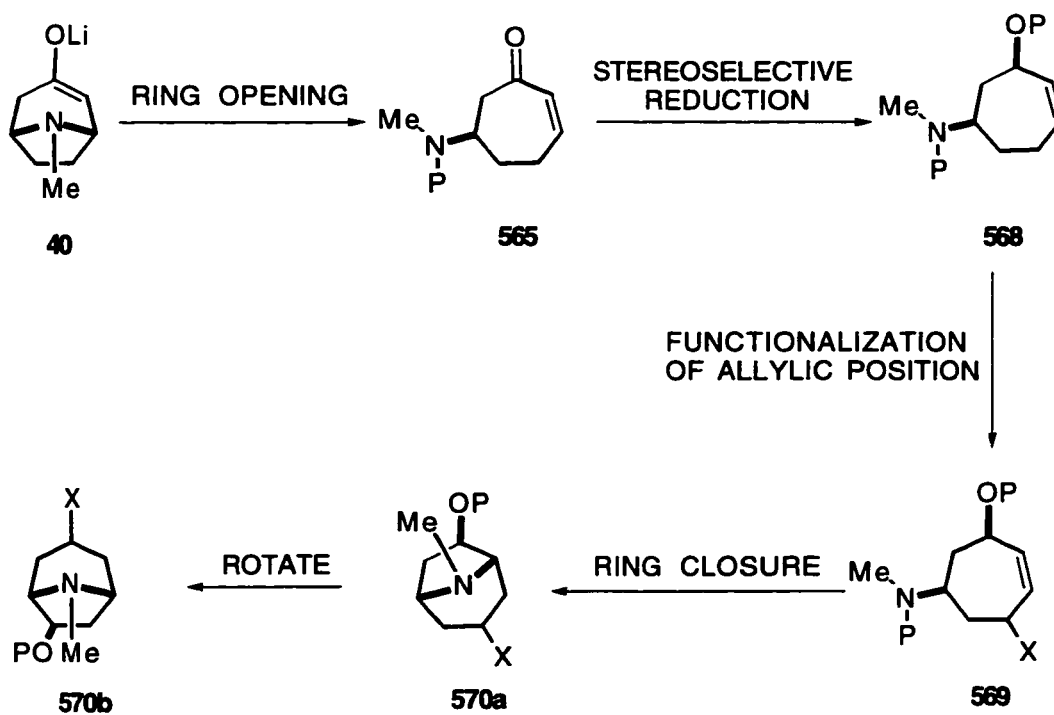
Scheme 93
