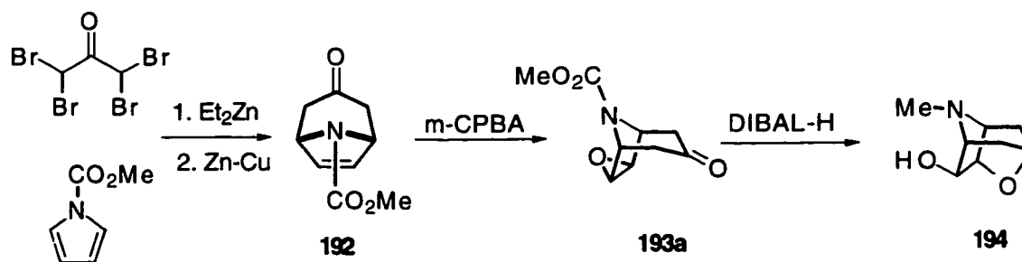
Scheme 36
