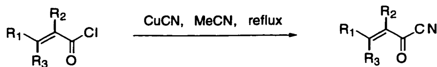
Scheme 81
