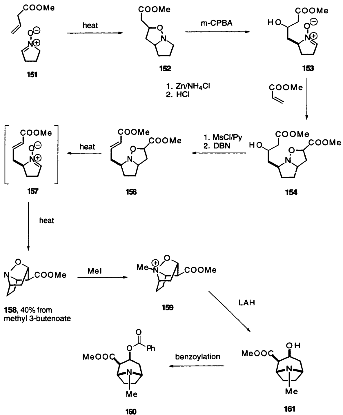
Scheme 28
