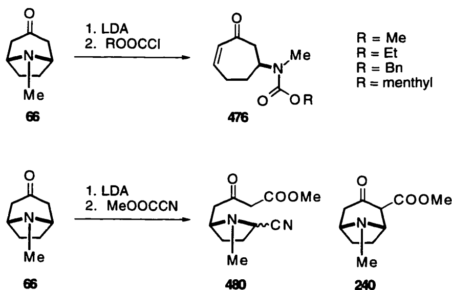
Scheme 78
