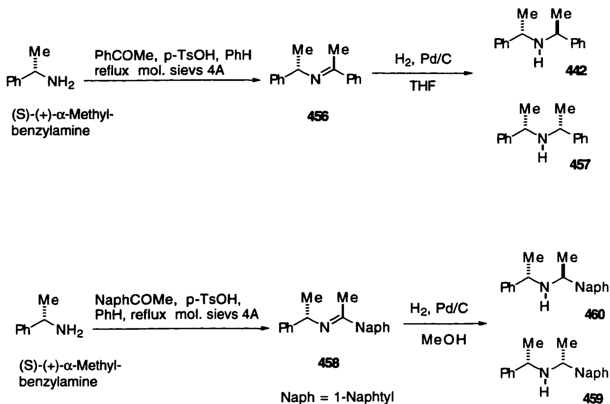
Scheme 68
