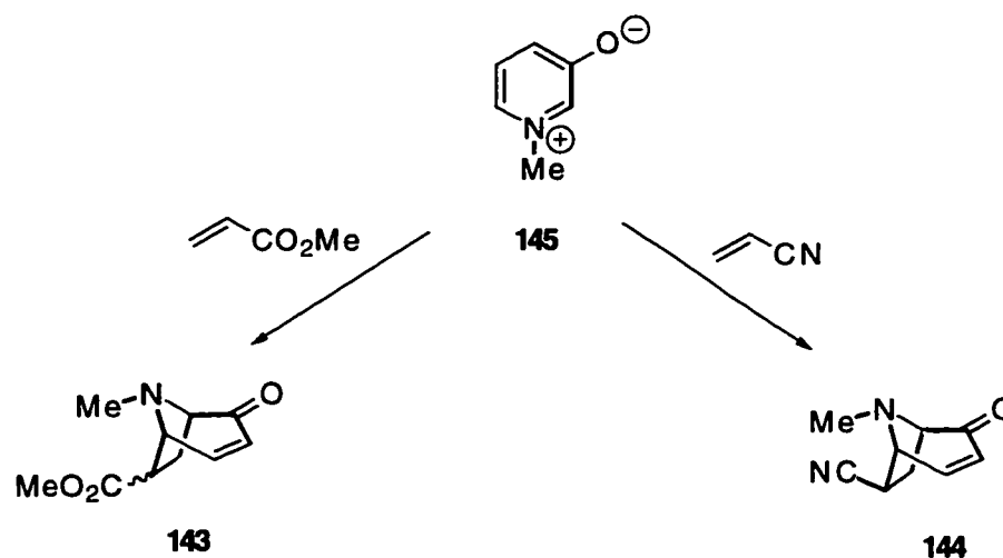
Scheme 26
