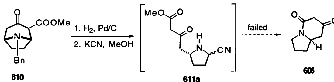
Scheme103
