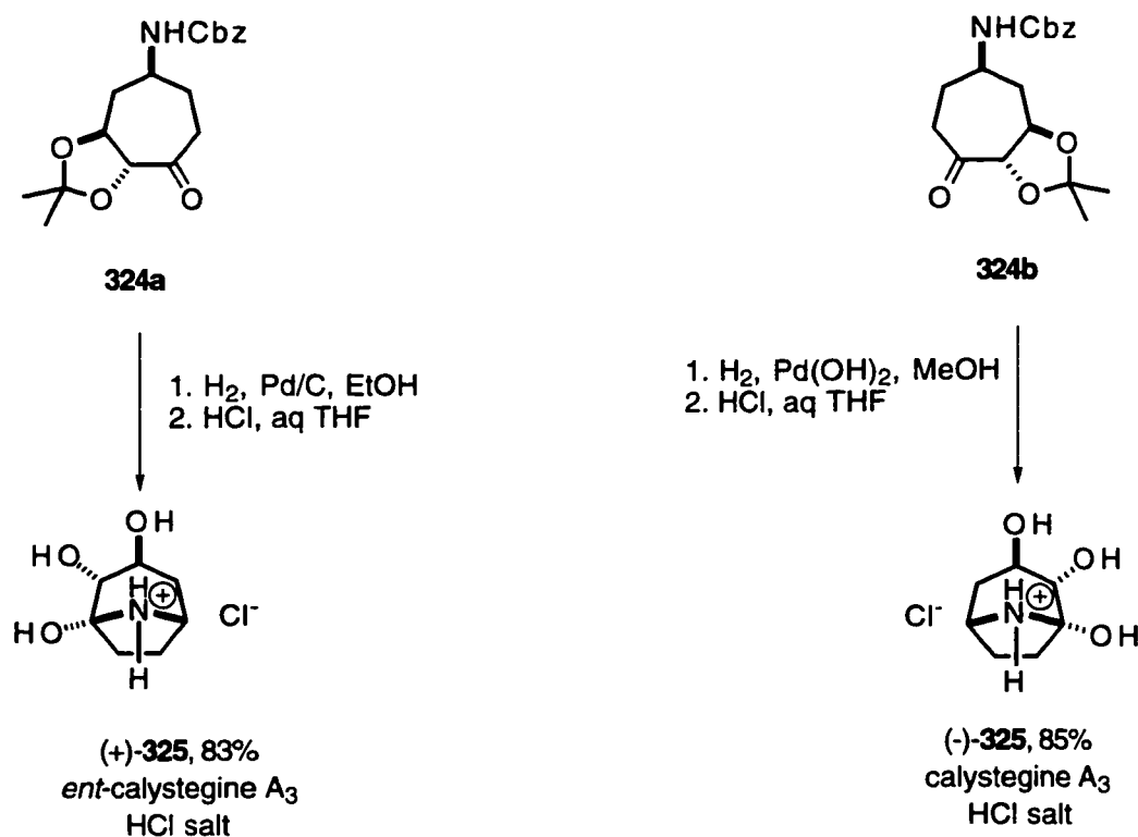
Scheme 62
