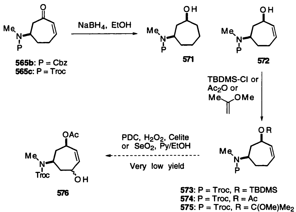
Scheme 94
