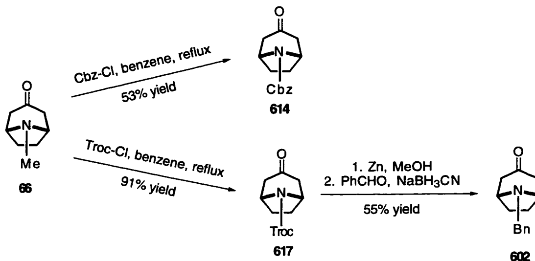
Scheme 104
