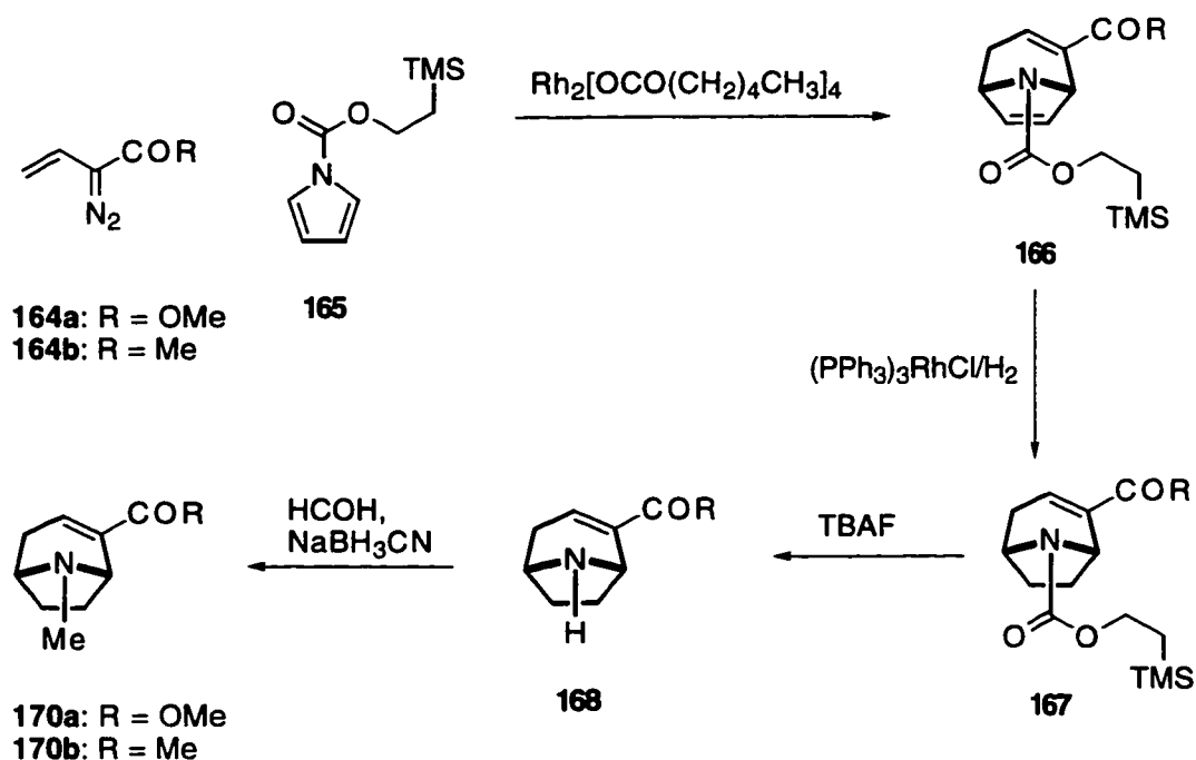
Scheme 30
