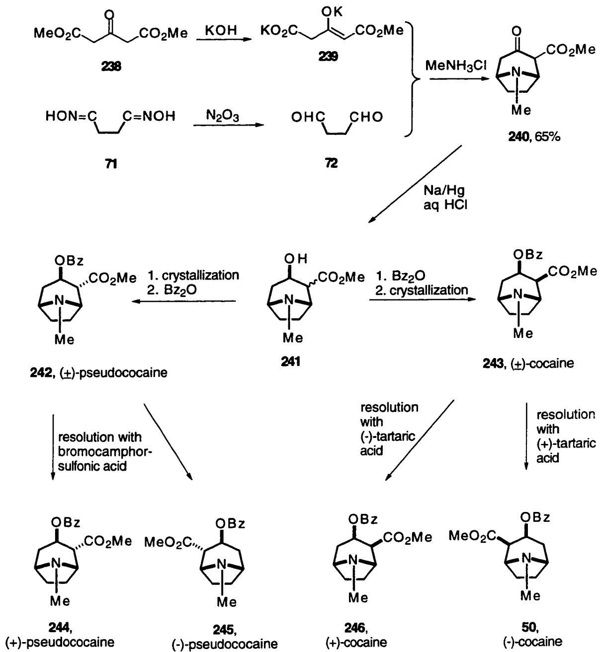
Scheme 44
