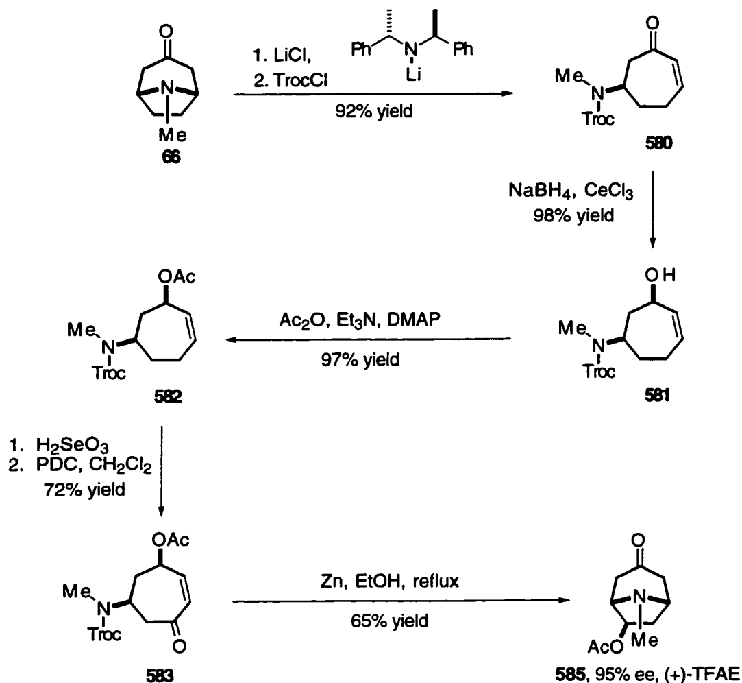
Scheme 96
