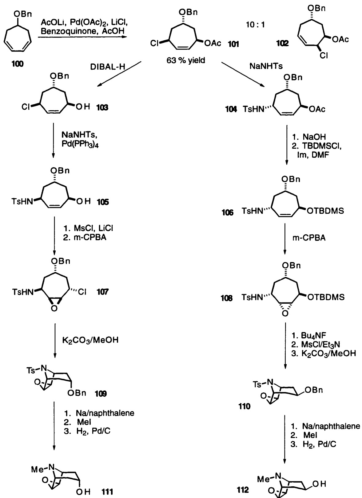
Scheme 20
