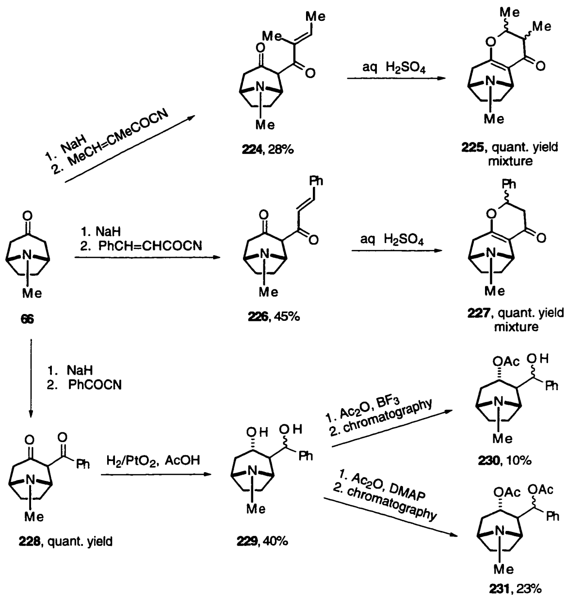
Scheme 42
