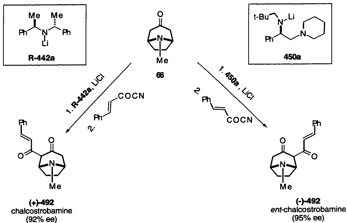
Scheme 83
