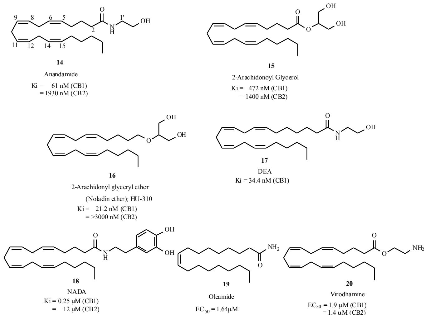
Fig. (3). Endogenous CB1 agonists.
