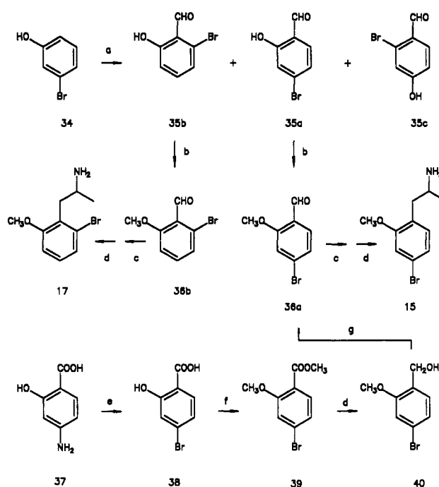
Scheme I a
