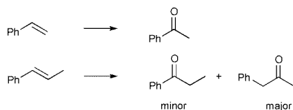
Scheme 1 Reagents and conditions: PdCl 2 (0.1), DMF, H 2 O, CuCl, O 2 , 50 °C.
