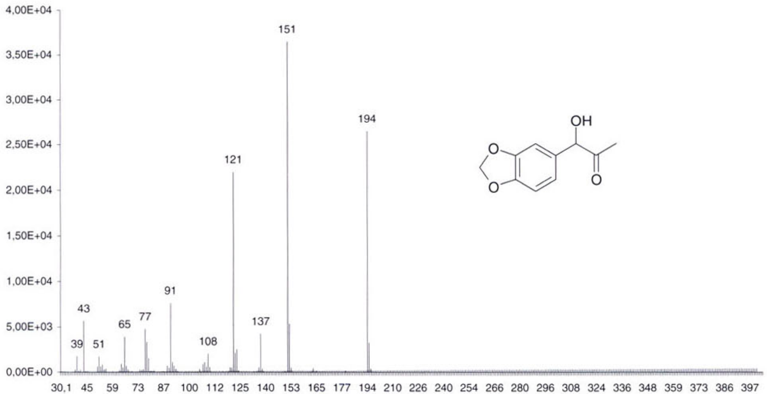
Fig. 12. Mass spectrum of 1-hydroxy-1-(3,4-methylenedioxyphenyl)-2-propanone (compound 6 in Table 1).
