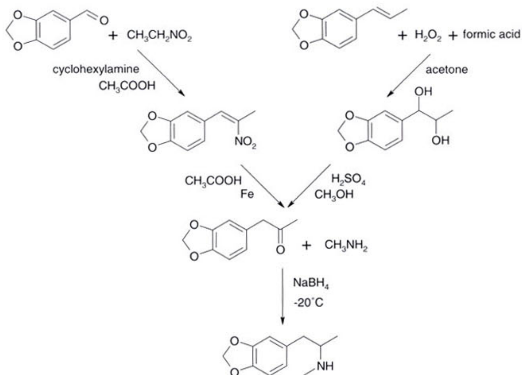
Fig. 1. Scheme of synthesis of MDP-2-P and MDMA.
