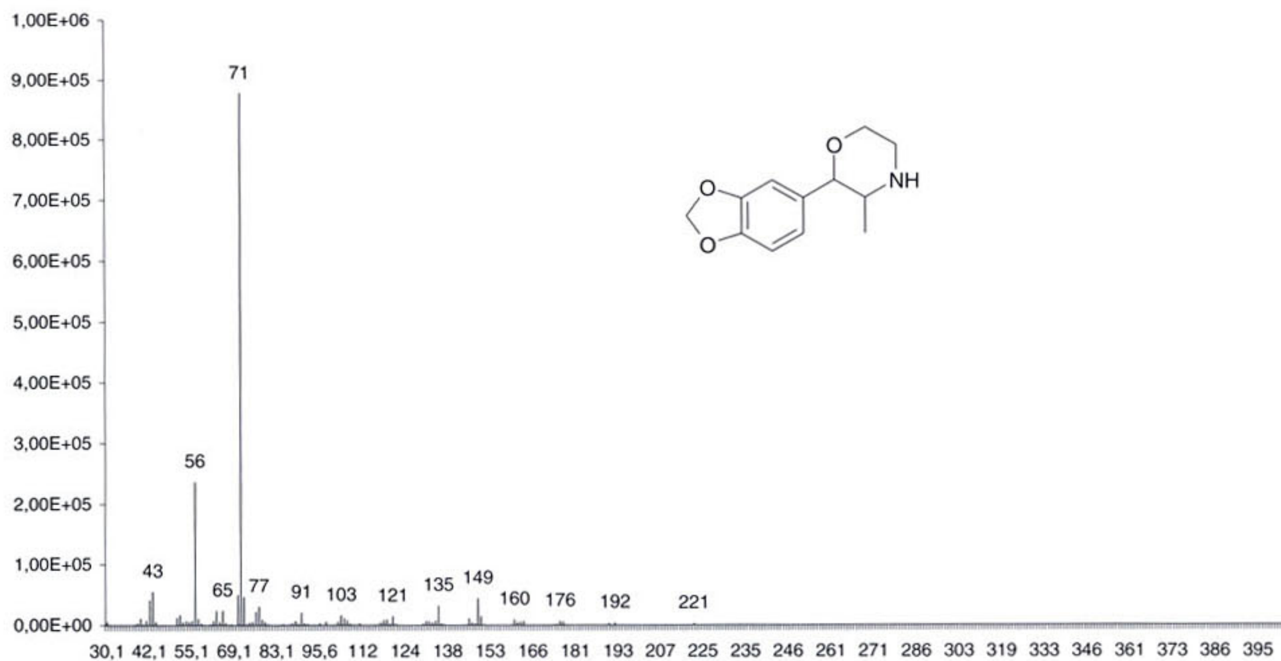
Fig. 9. Mass spectrum of 2-Methyl-(6,7-methylenedioxyphenyl)-3-methylmorpholine (compound 14 in Table 1).
