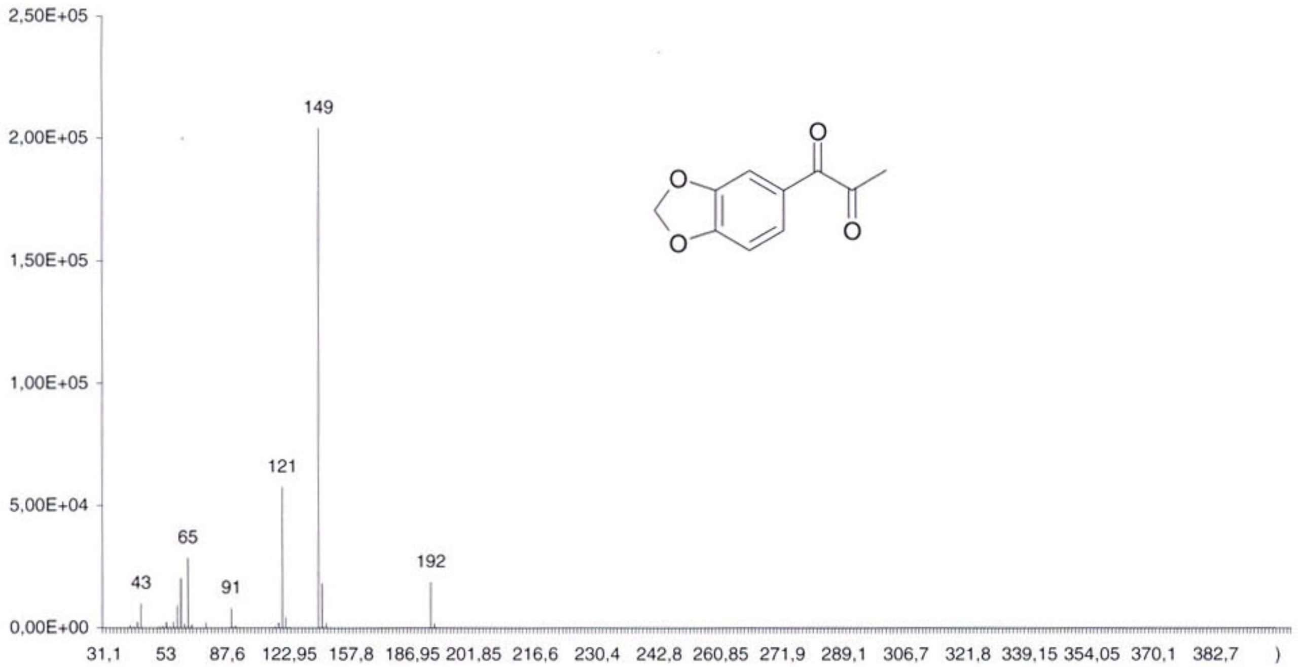
Fig. 11. Mass spectrum of 1-(3,4-methylenedioxyphenyl)-1,2-propanedione (compound 5 in Table 1).
