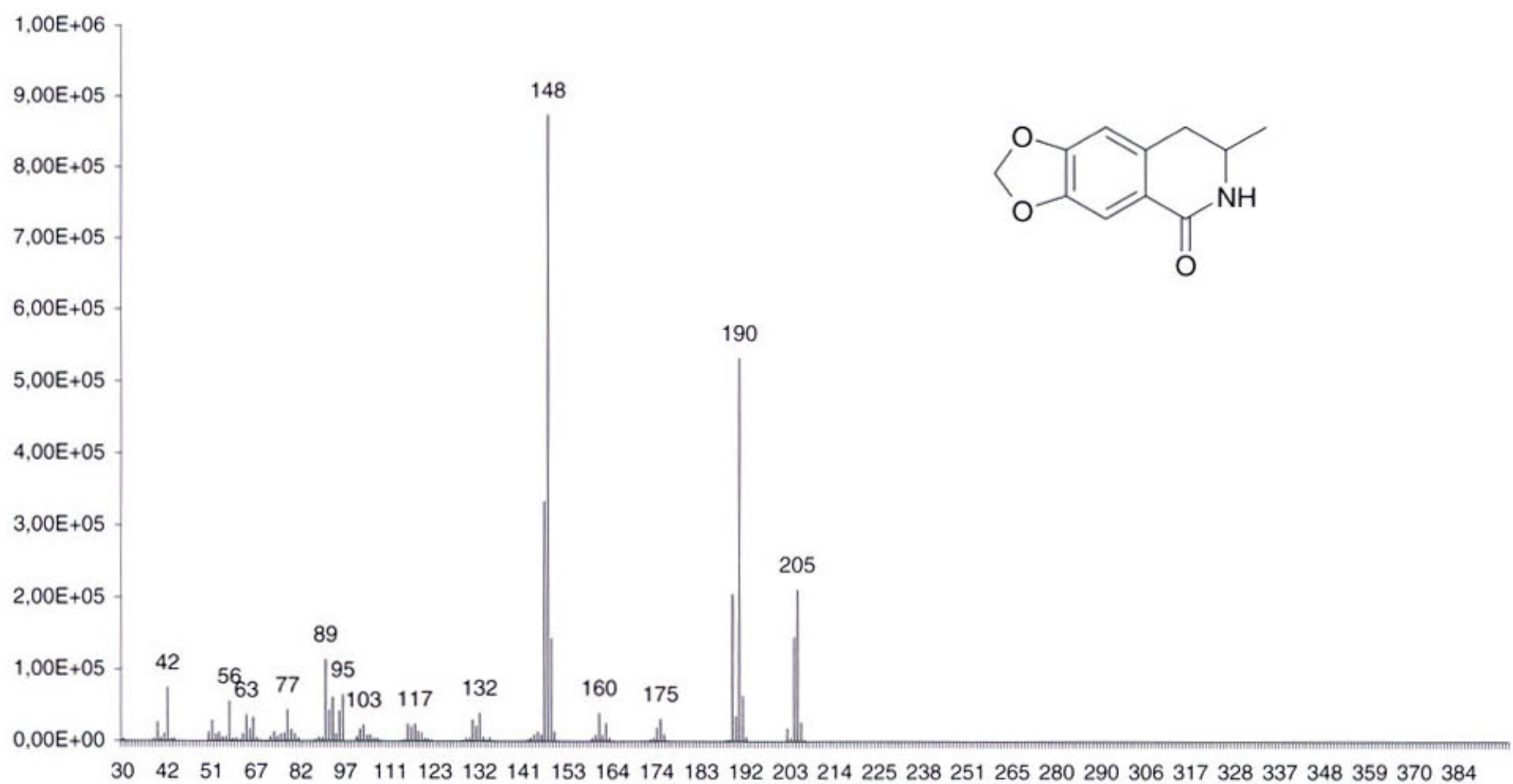
Fig. 8. Mass spectrum of 3-methyl-6,7-methylenedioxy-3,4-dihydroisoquinolin-1(2H)-one (compound 13 in Table 1).
