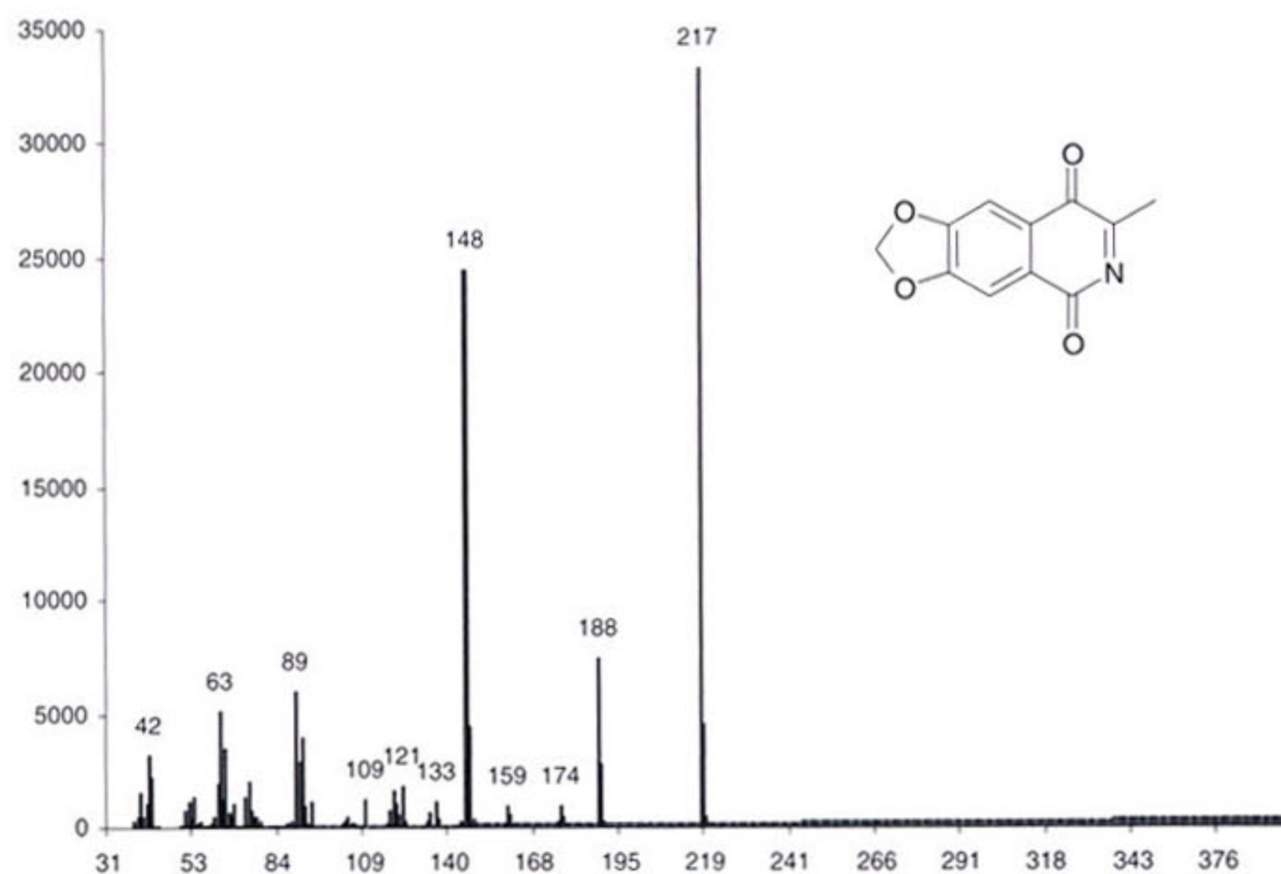
Fig. 3. Mass spectrum of 3-methyl-6,7-methylenedioxyisoquinoline-1,4-dione (compound 15 in Table 1).
