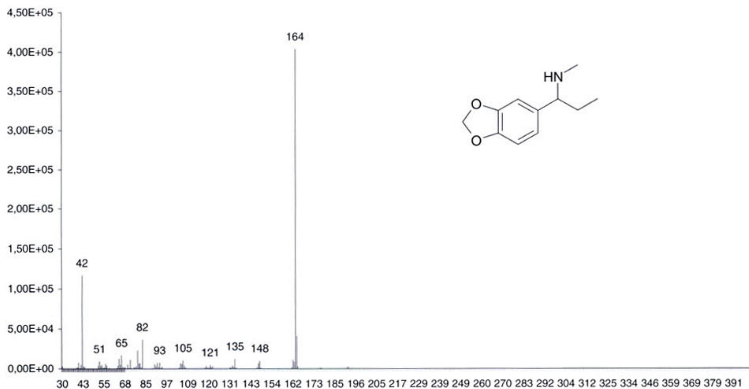
Fig. 10. Mass spectrum of N -methyl-1-(3,4-methylenedioxyphenyl)-1-propanamine (compound 17 in Table 2).
