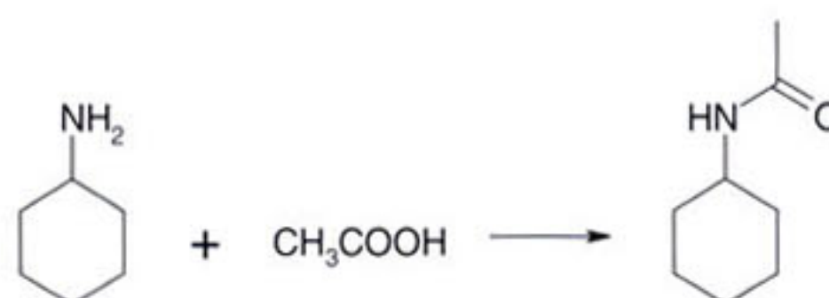
Fig. 2. One of the side-reactions occurring during the synthesis of MDP-2-nitropropene.
