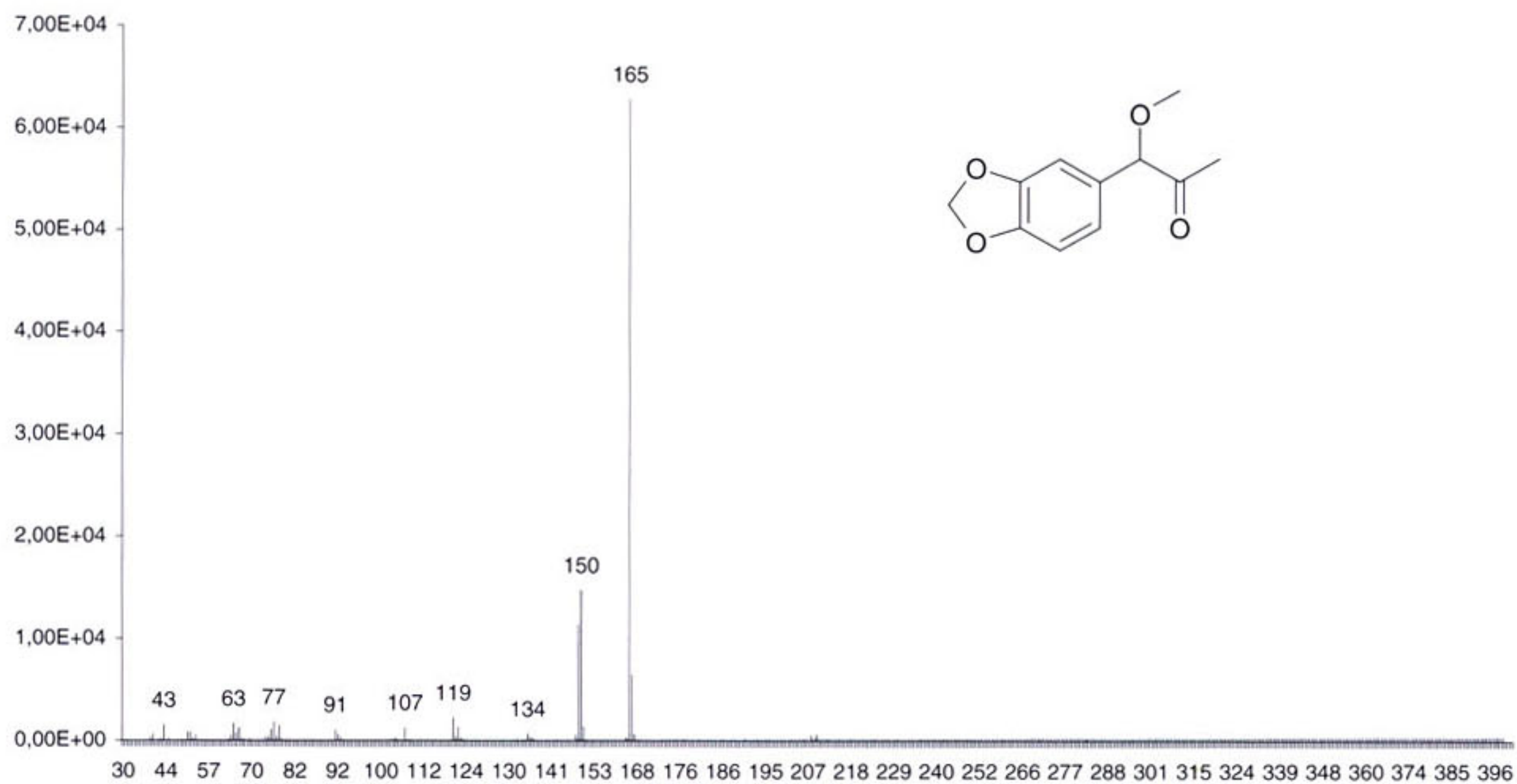
Fig. 7. Mass spectrum of 1-methoxy-1-(3,4-methylenedioxyphenyl)-2-propanone (compound 11 in Table 2).
