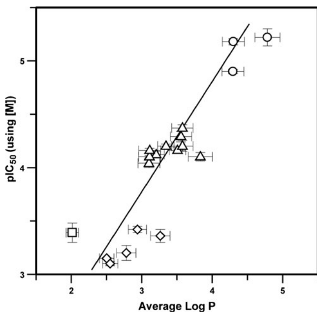
Fig. 6 Calculated lipophilicities of MDMA and analogues versus cytotoxic performance. Relationship between average log P \pm SEM and pIC_{50} \pm SEM for MDMA ( \square ), alkyl \alpha -substituted analogues 1–5 ( \diamond ), monocyclic aromatic \alpha -substituted analogues 6–15 ( \Delta ) and polycyclic aromatic \alpha -substituted analogues 16–18 ( \circ ). The curve was fitted to all data points shown using weighted linear regression that gave an r^2 value of 0.88
