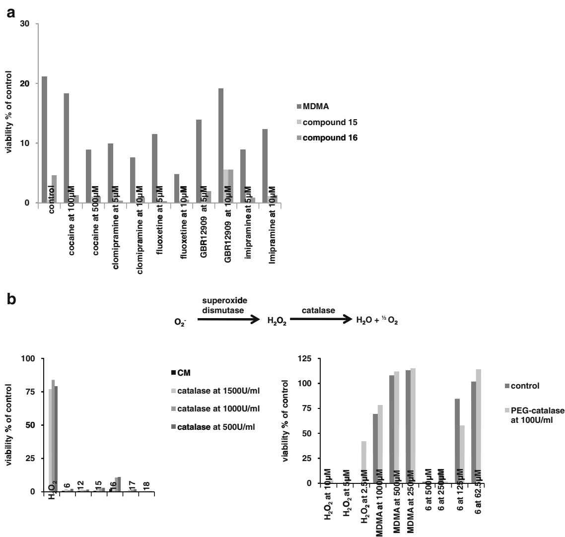
Fig. 5 Investigation of potential pathways through which MDMA analogues elicit cytotoxicity in L3055 cells. a Impact of monoamine transporter (MAT) inhibitors. L3055 cells at 10^5 /ml were pre-incubated with MAT inhibitors for 1 h before adding MDMA or compounds 15 and 16 at 125 \mu M and 31.25 \mu M respectively then culturing for 20 h prior to assessing cell viability as in Fig. 1c; b Influence of scavenging extracellular ROS with catalase. L3055 cells at 10^5 /ml were pre-treated with catalase at concentrations shown for 1 h before adding
