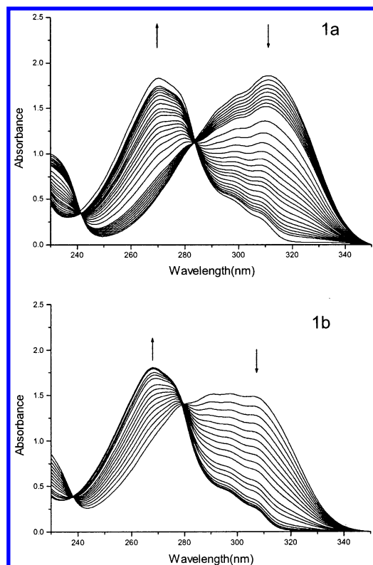
FIGURE 1. Spectral profile during the bromodecarboxylation of 4-OMeC 6 H 4 CH=CHCO 2 H, 1 , to 4-OMeC 6 H 4 CH=CHBr, 1a : (a) Et 3 N as catalyst in CH 2 Cl 2 ; (b) LiOAc as catalyst in MeCN–H 2 O (97:3 v/v).
