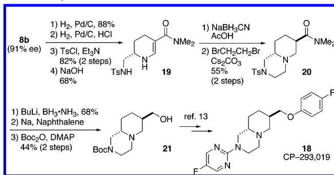
Scheme 1. Catalytic Enantioselective Synthesis of Intermediate for CP-293,019
