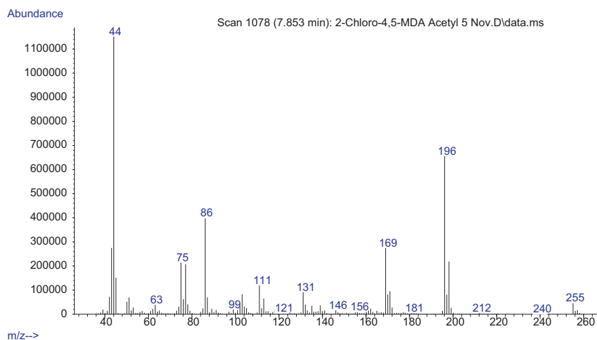
Fig. 5. Mass spectrum of N-acetyl-2-chloro-4,5-methylenedioxyamphetamine (Ac-2-Cl-4,5-MDA).
