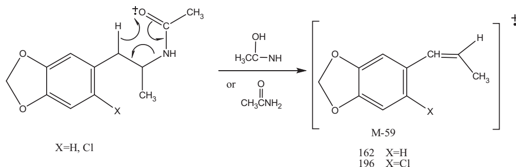
Fig. 8. Origin of the M-59 ion in N-acetyl derivatives of MDA and 2-chloro-4,5-methylenedioxyamphetamine [18].
