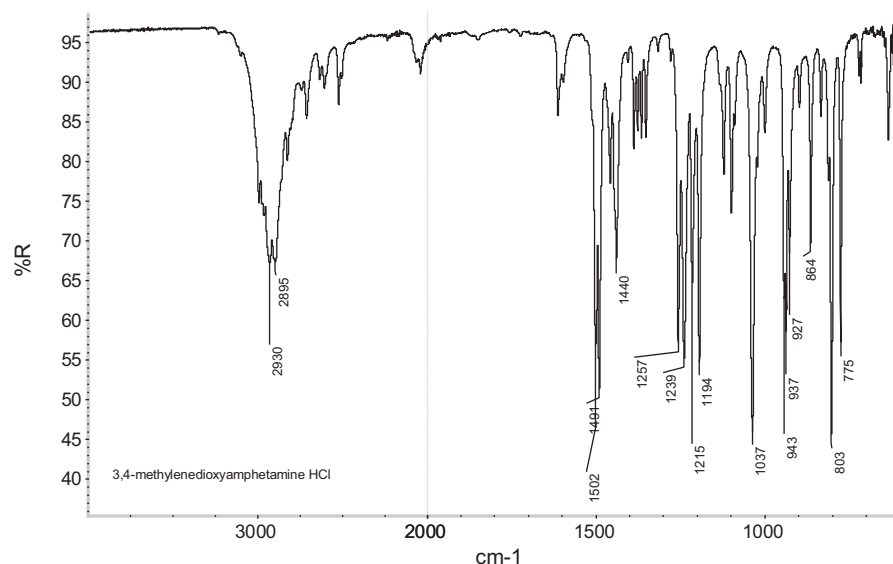
Fig. 16. IR (ATR) of 3,4-methylenedioxyamphetamine HCl (MDA HCl).
