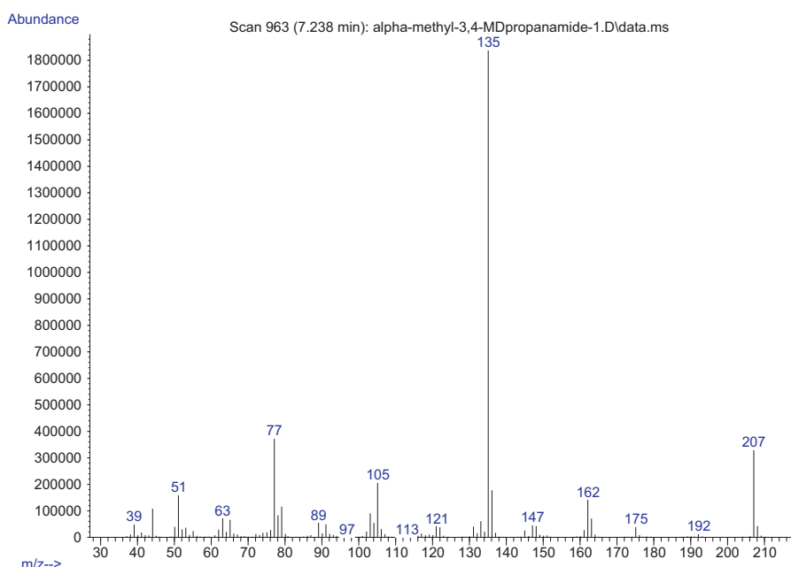
Fig. 7. Mass spectrum of \alpha -methyl-3,4-methylenedioxyphenylpropanamide (MMDPPA).
