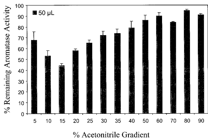
FIGURE 4 Step gradient fractionation of white button ( Agaricus bisporus ) mushroom extract. Fractionation of 5 mL of the lyophilized and reconstituted crude white button mushroom extract ( 10\times_{\text{H}_2\text{O}} ) was performed using a step gradient on Sep-Pak C18 solid phase cartridges. Dose response data were quantified using the human placental microsomal assay. The assay was done in triplicate for each dose at each eluted fraction. The data are expressed as the percentage of activity remaining compared with the untreated control, which is expressed as 100%.
