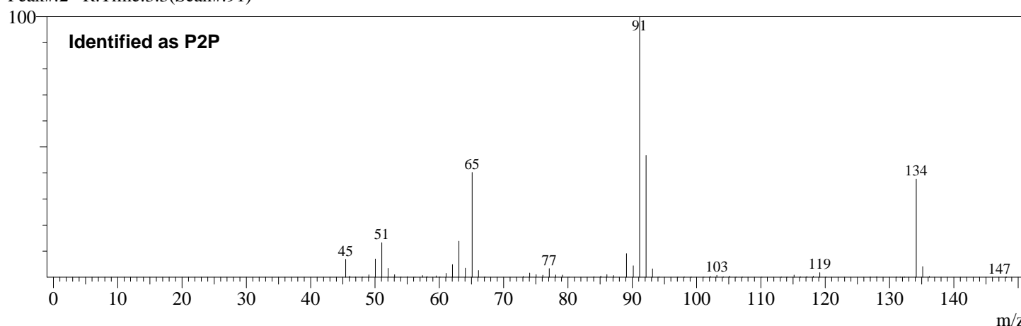
Peak#:2 R.Time:3.3(Scan#:91)
