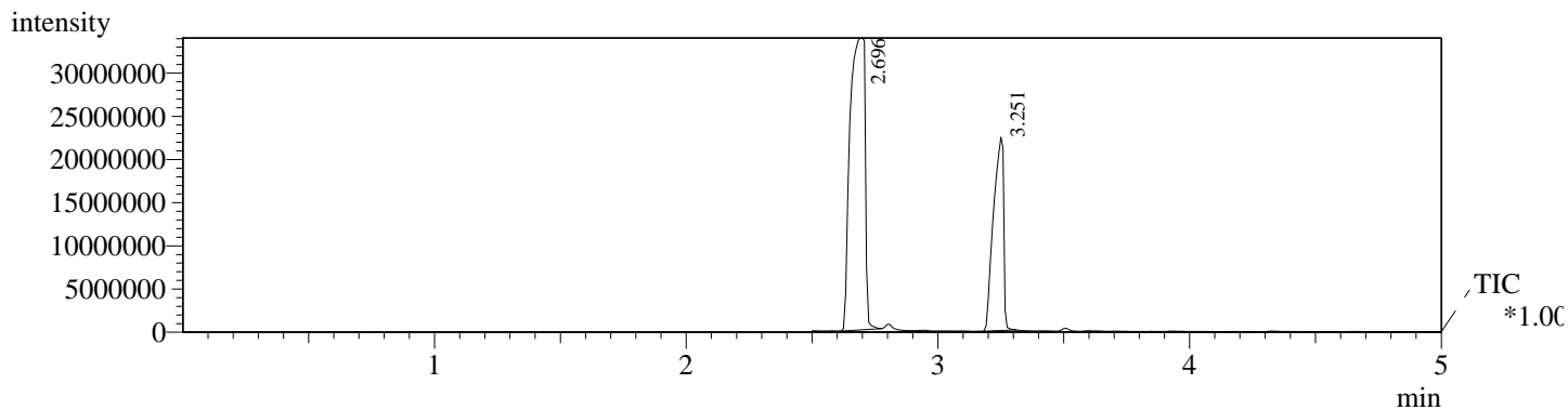
Peak#:1 R.Time:2.7(Scan#:25)
