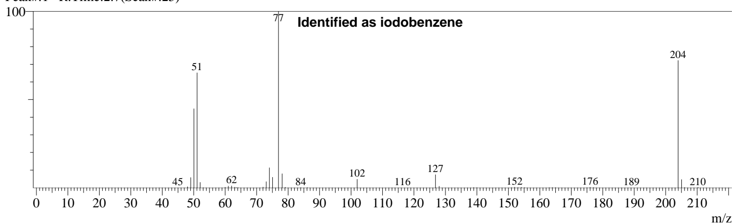
Peak#:2 R.Time:3.3(Scan#:91)
