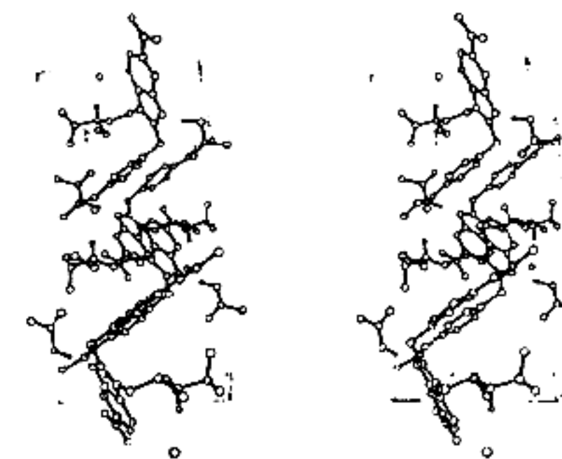
Fig. 3. Stereoscopic view of the packing.
