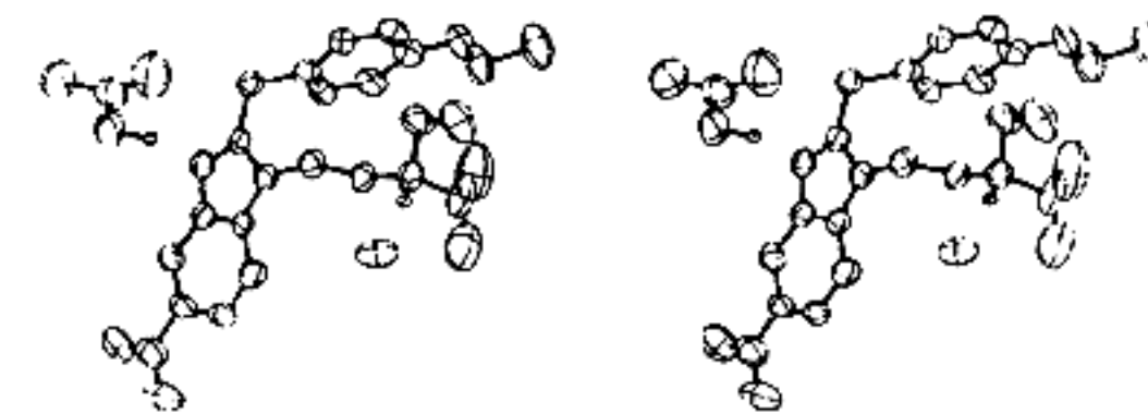
Fig. 2. Stereoscopic view (Johnson, 1965) of the molecule with 50% probability thermal ellipsoids.
