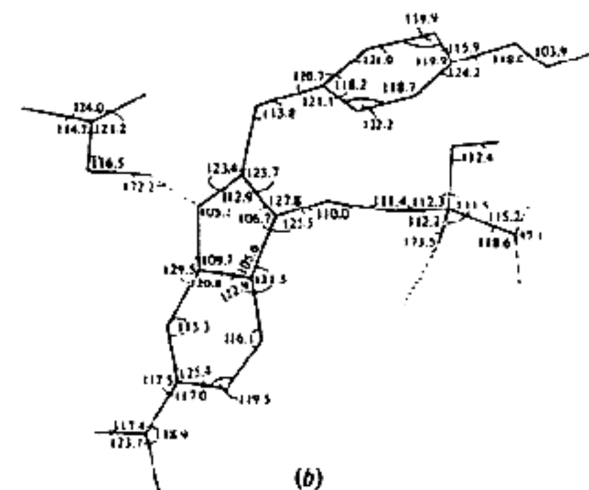
Fig. 1. (a) Bond distances (Å) and (b) angles (°). The average e.s.d.'s for the lengths are 0.009 Å and for angles 0.6° except for the terminal ethyl groups for which e.s.d.'s range between 0.026-0.012 Å and 0.8-1.3°.
