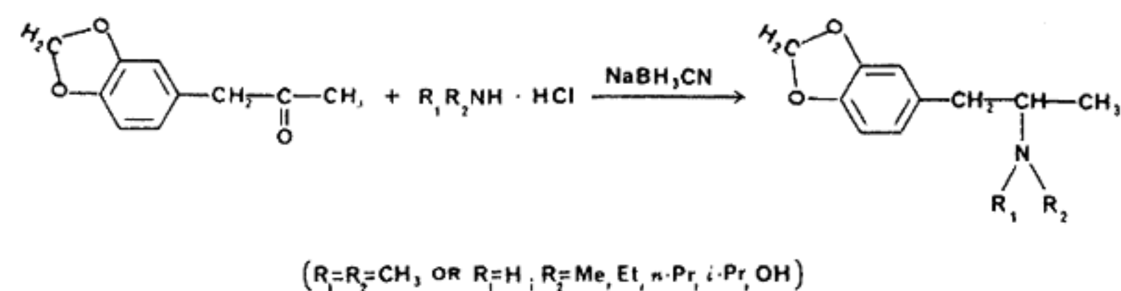
FIG. 2—Synthesis scheme for N -substituted MDA analogs.
