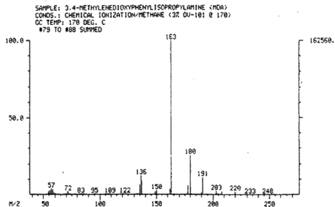
FIG. 10—Chemical ionization mass spectra for MDA and related compounds.
