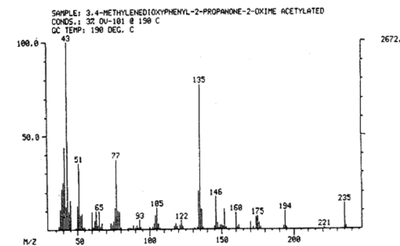
FIG. 11—Mass spectra of acetylated MDA, acetylated N -hydroxy MDA, and acetylated MDP-2-P-oxime.
