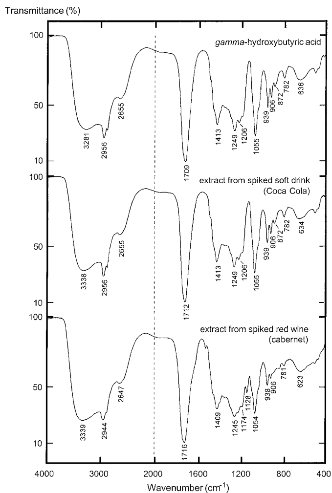
FIG. 5—Infrared transmission spectra ( 4\text{ cm}^{-1} resolution) for gamma -hydroxybutyric acid and residues extracted from two spiked beverages (Coca Cola® and red wine), each examined neat between KBr disks.
