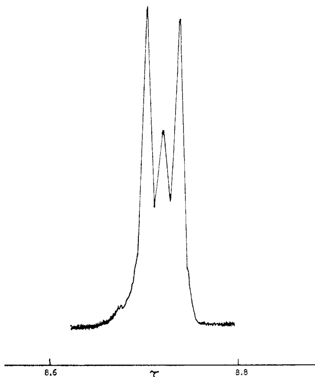
Figure 1. Pmr spectrum of [C 5 Me 5 RhCl 2 ] 2 (diphos) in CDCl 3 in the methyl region.
